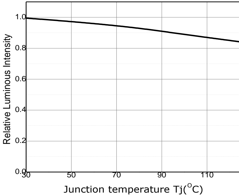
Fig 6. Relative Light Output vs. Junction Temperature, I_F=40\text{mA}
