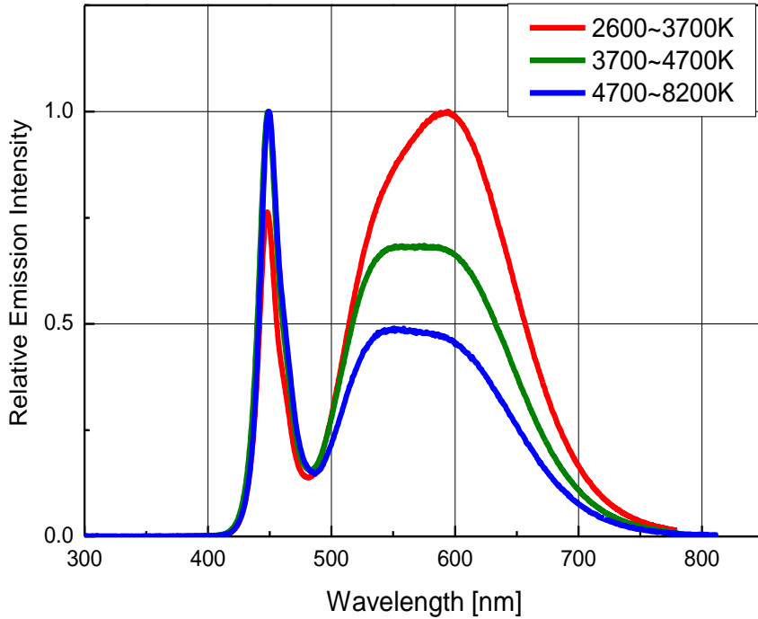
Fig 1. Color Spectrum, T_a = 25^\circ\text{C} , RH30%, I_F=40\text{mA}
