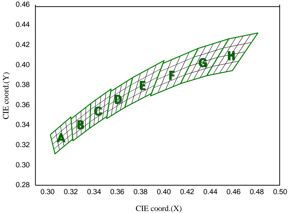
CIE Chromaticity Diagram, T_a=25^{\circ}\text{C} , I_f=40\text{mA}
