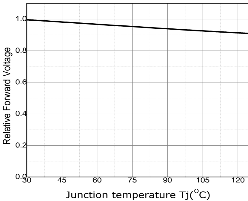
Fig 7. Junction Temperature vs. Relative Forward Voltage, I_F=40\text{mA}
