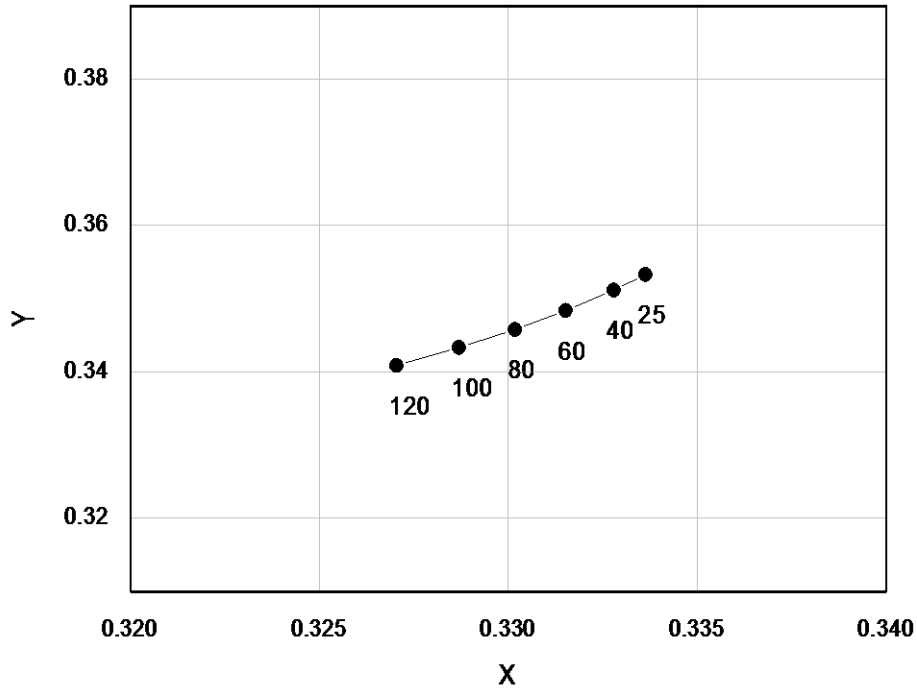
Fig 8. Chromaticity Coordinate vs. Junction Temperature, I_F=40mA
