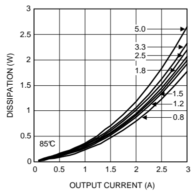
Figure 12. Dissipation 8-V Input at 85°C
