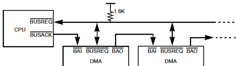
Figure 31. Bus-Requesting Daisy-Chain
