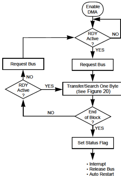
Figure 22. Burst Mode
