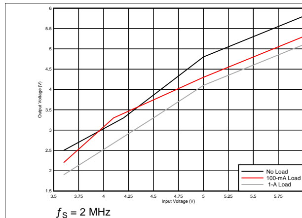
Figure 1. Buck-Regulator Output Voltage
