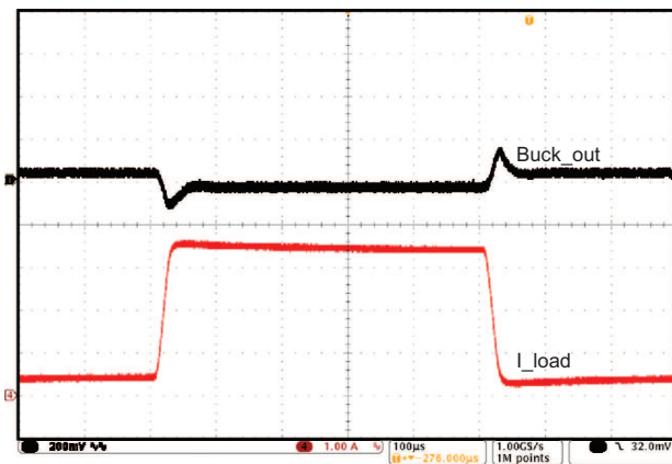
Figure 18. Buck Regulator Output at Load Transient (200 mA to 3 A, Buck Output Voltage = 5 V, f_s = 2 MHz)
