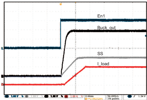
Figure 19. Buck-Regulator Startup Operation
