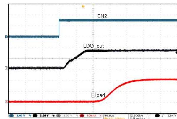
Figure 20. LDO Regulator Startup Operation
