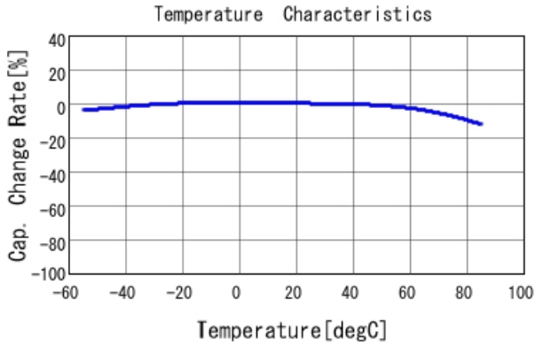
■ GRM033R60G225ME47 C-Temp. capchange, DCO. 0V, ACO. 2Vrm
