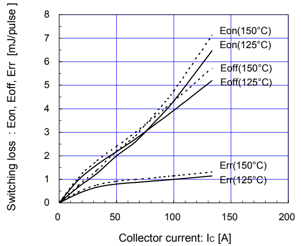
[ Inverter ]
