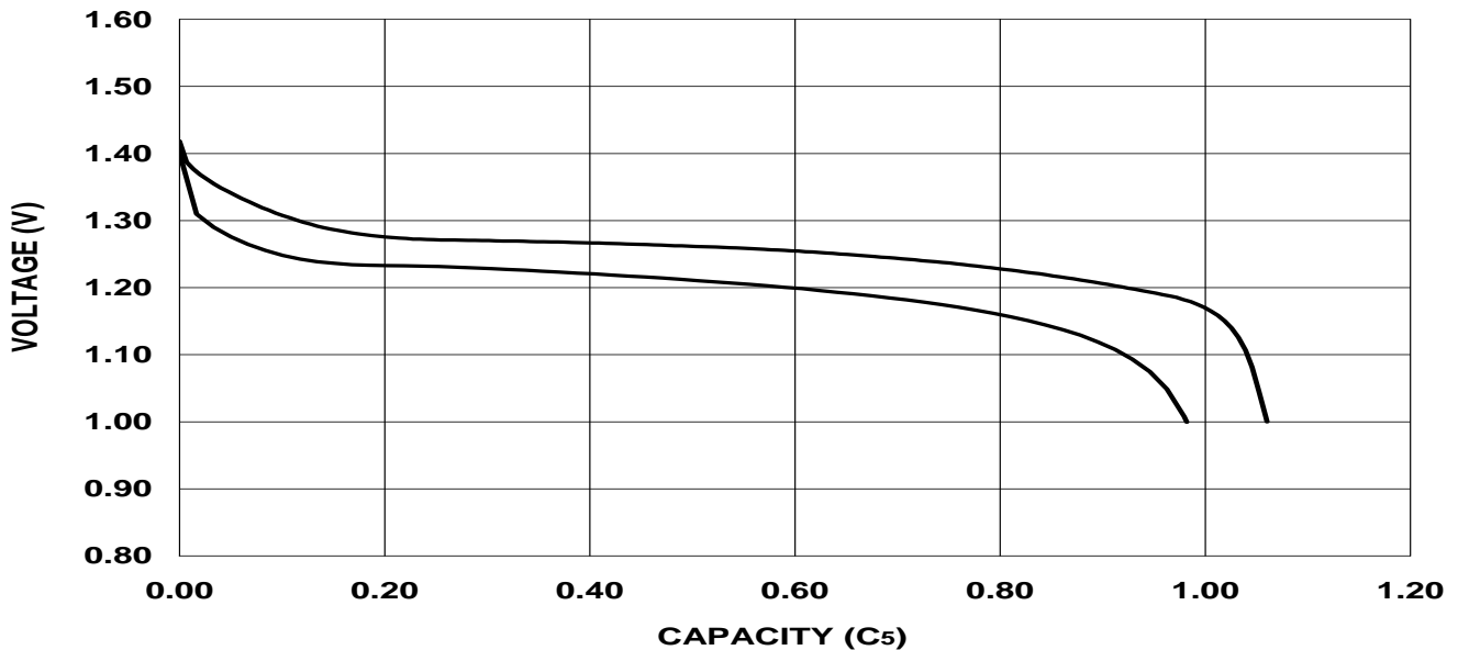
DISCHARGE CHARACTERISTICS OF BPI-48AA1000 CELL
