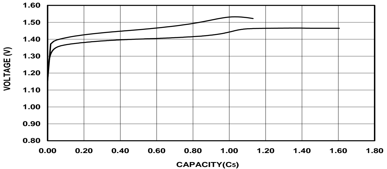
CHARGING CURVE OF BPI-48AA1000 CELL
