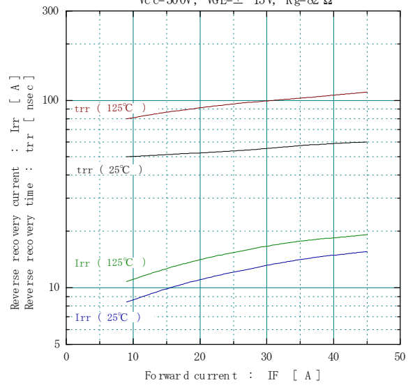
[ Inverter ] Reverse recovery characteristics (typ.) Vc=300V, VGE=±15V, Rg=82Ω
