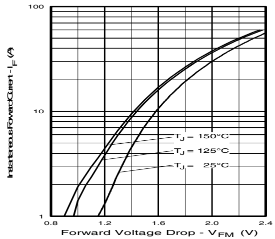
Fig. 10 - Maximum Diode Forward Characteristics t_p = 80\mu s
