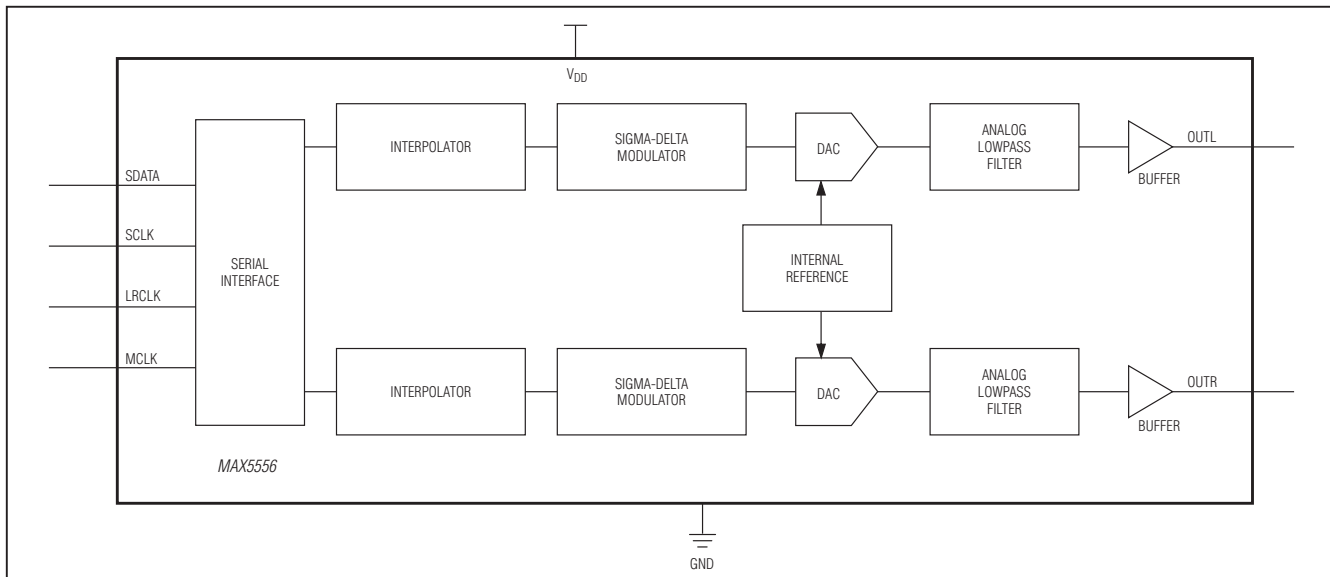
Figure 2. Functional Diagram
