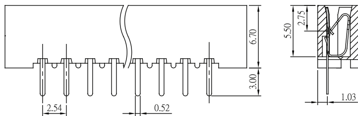
Recommended PCB Layout (PCB TOLERANCE ±0.05)
