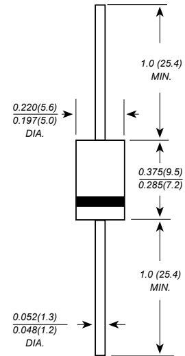
Dimensions in inches and (millimeters) DO-201AD
