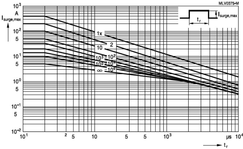
CU3225K50G2 ... K300G2
