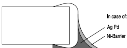
Good solder joint
