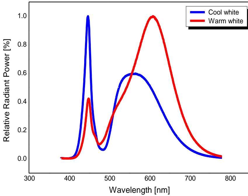
Fig 1. Color Spectrum, T_a = 25^\circ\text{C} , I_F = 350\text{mA} , \text{RH}30\%
