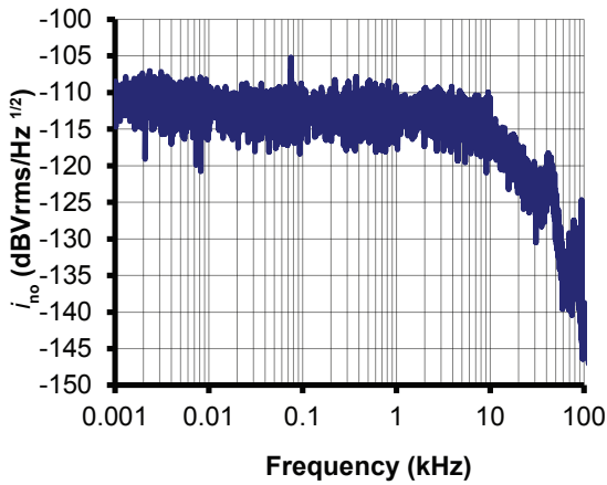
Figure 13: Typical noise current density i_{no} with R_M = 50 \Omega
