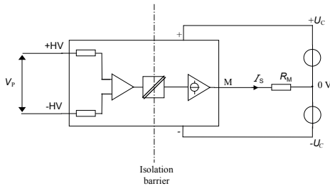
Figure 16: standard characterization schematics for voltage output transducers ( R_M = 50 \Omega unless otherwise noted)
