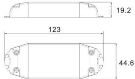
Dimension in mm
