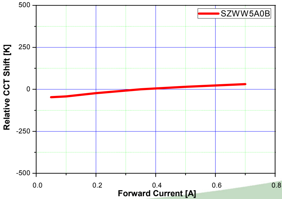
Forward Current vs. CCT, Ta=25°C
