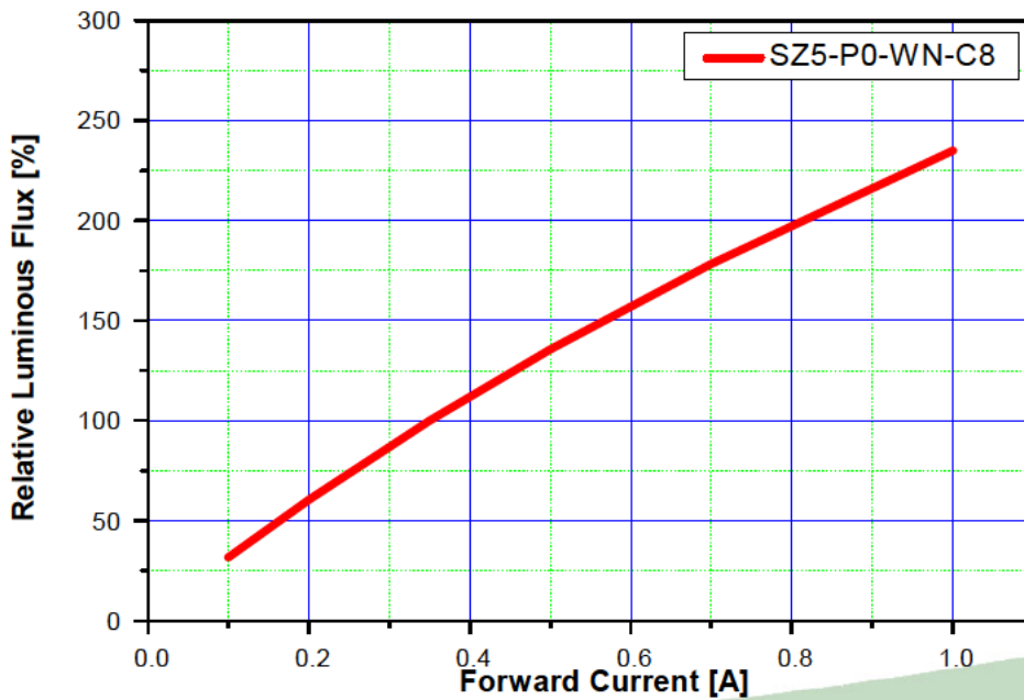
Forward Current vs. Normalized Relative Luminous Flux, Ta=25°C
