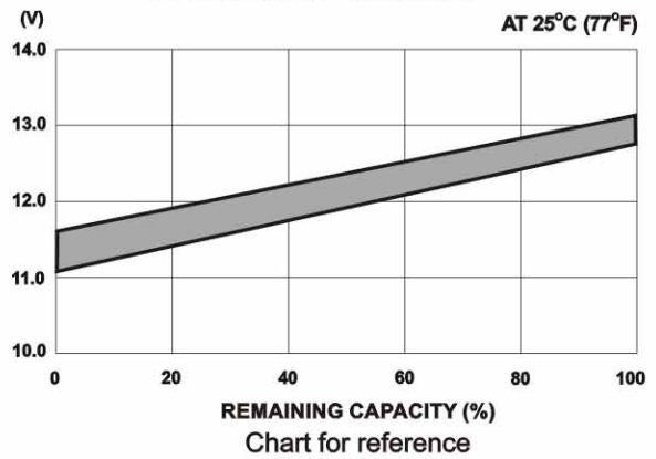
OPEN CIRCUIT VOLTAGE VS REMAINING CAPACITY
