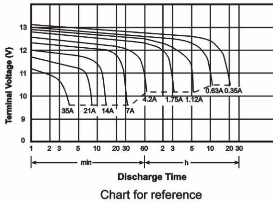
Discharge Characteristics 25 °C ( 77 °F)
