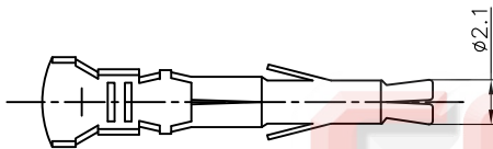
Male TERMINAL
