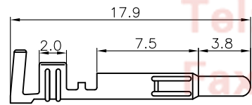
Male TERMINAL
