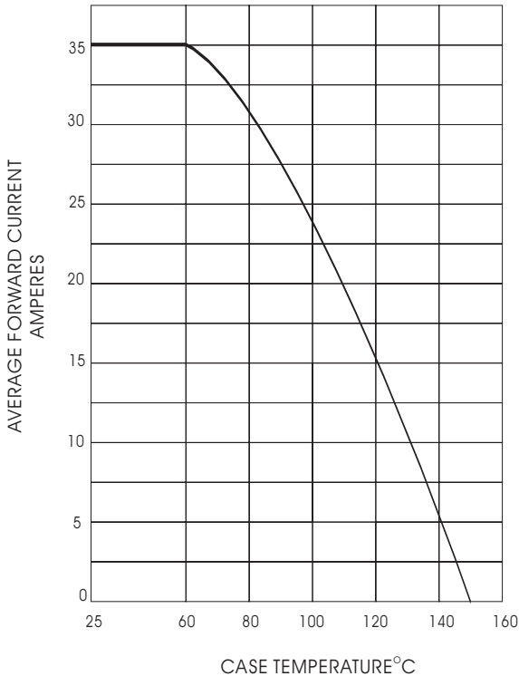
Fig. 1- OUTPUT CURRENT VS. CASE TEMPERATURE RESISTIVE OR INDUCTIVE LOAD T_J = 150^{\circ}C
