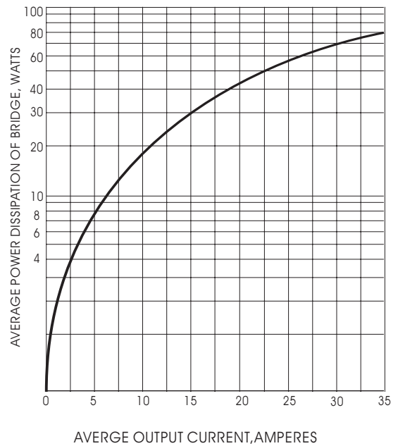
Fig. 4- POWER DISSIPATION VS. AVERAGE OUTPUT CURRENT RESISTIVE OR INDUCTIVE LOAD T_J = 150^{\circ}C
