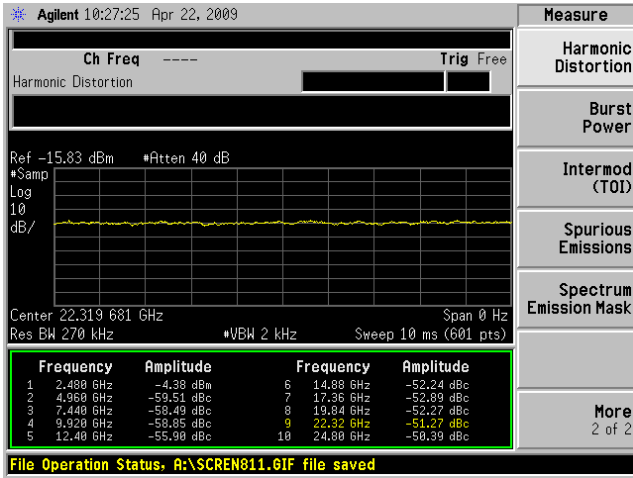
/ Frequency 2.480 GHz
