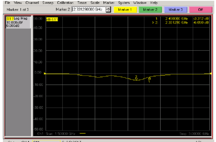
/ S11dB (Die Model)
