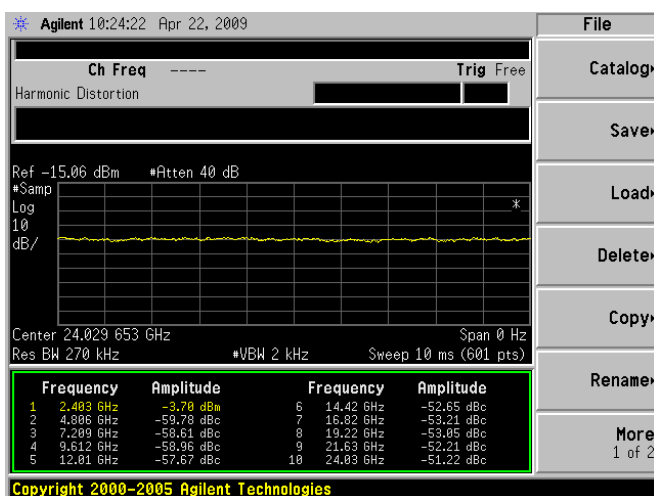
/ Frequency 2.403 GHz
