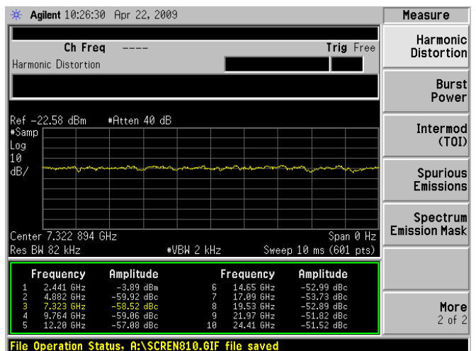
/ Frequency 2.441 GHz
