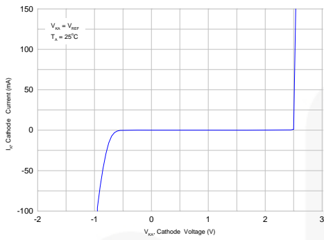
Figure 5. Cathode Current vs. Cathode Voltage
