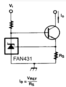
Figure 18. Constant-Current Sink
