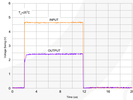
Figure 10. Pulse Response
