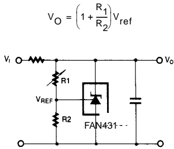
Figure 14. Shunt Regulator
