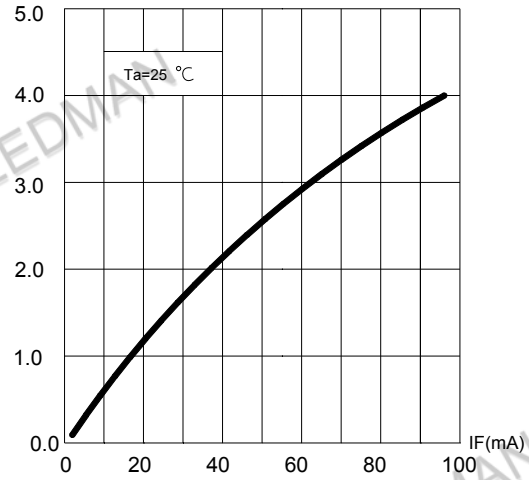
Fig.2 Relative Luminous Intensity vs. Forward Current Domi WL=590nm
