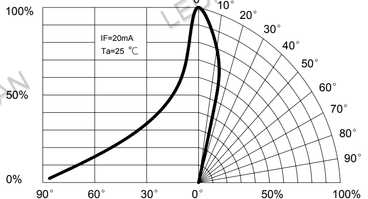
Fig.6 Relative Luminous Intensity vs. Radiation Angle
