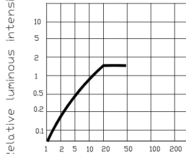
Fig.2 Luminous Intensity vs Forward Current
