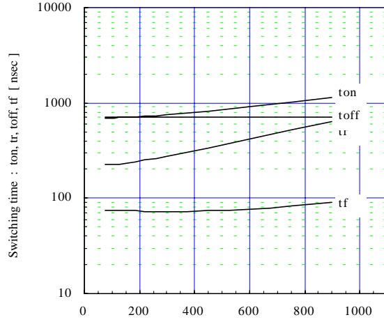
Switching time vs. Collector current (typ.) V_{cc}=300V, V_{GE}=\pm 15V, R_g=4.7\Omega, T_j=125^\circ C
