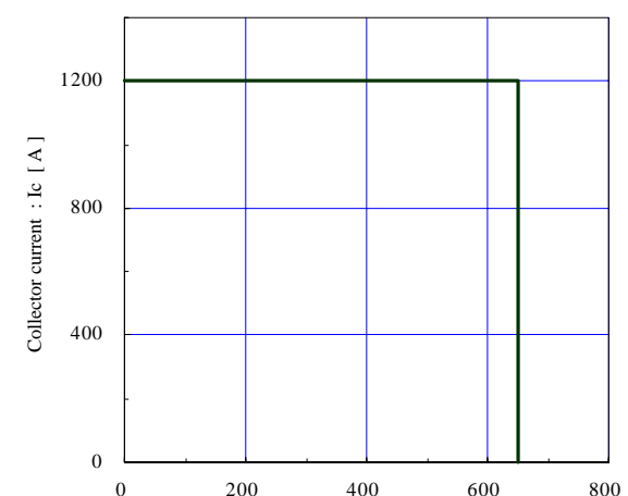
Reverse bias safe operating area (max.) +V_{GE}=15V, -V_{GE} \le 15V, R_g \ge 4.7\Omega, T_j \le 125^\circ C
