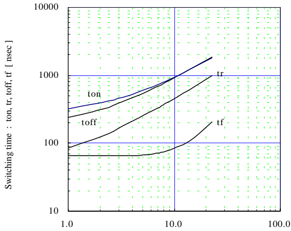
Switching time vs. Gate resistance (typ.) V_{cc}=300V, I_c=600A, V_{GE}=\pm 15V, T_j=25^\circ C
