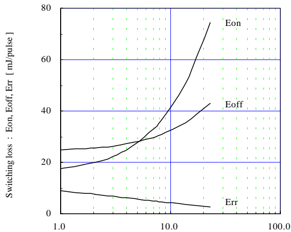
Switching loss vs. Gate resistance (typ.) V_{cc}=300V, I_c=600A, V_{GE}=\pm 15V, T_j=125^\circ C
