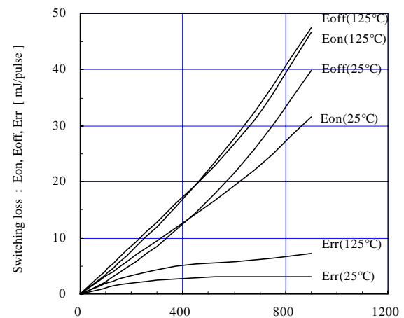
Switching loss vs. Collector current (typ.) V_{cc}=300V, V_{GE}=\pm 15V, R_g=4.7\Omega
