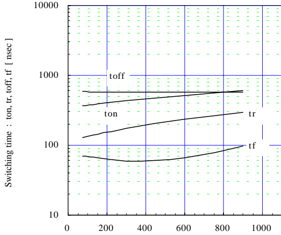
Switching time vs. Collector current (typ.) V_{cc}=300V, V_{GE}=\pm 15V, R_g=4.7\Omega, T_j=25^\circ C
