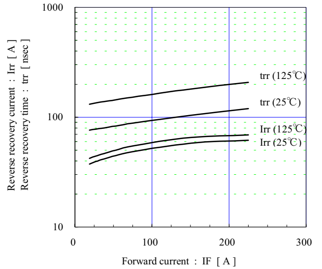
Reverse recovery characteristics (typ.) V cc =300V, V GE =±15V, R g =24Ω
