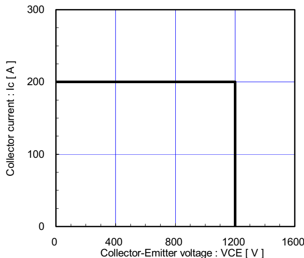
Reverse bias safe operating area (max.) +V_{GE}=15V, -V_{GE} \leq 15V, R_G \geq 5.6\Omega, T_J \leq 125^\circ C
