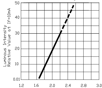
FORWARD VOLTAGE(VF)-VOLTS
