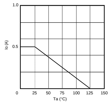
Fig.4 Derating curve
