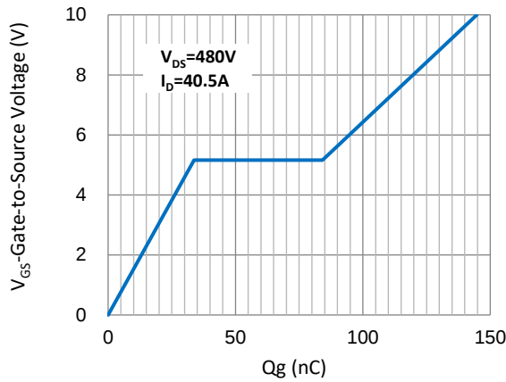
Fig.7 Gate-Charge Characteristics
