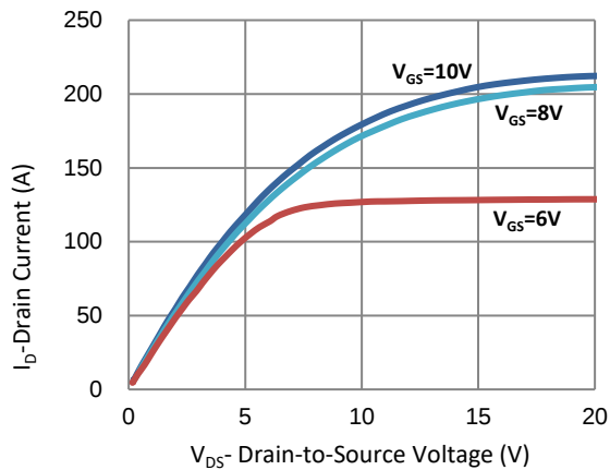
Fig.1 Output Characteristics
