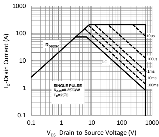
Fig.11 Maximum Safe Operating Area
