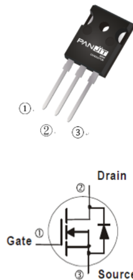
TO-247AD-3LD
