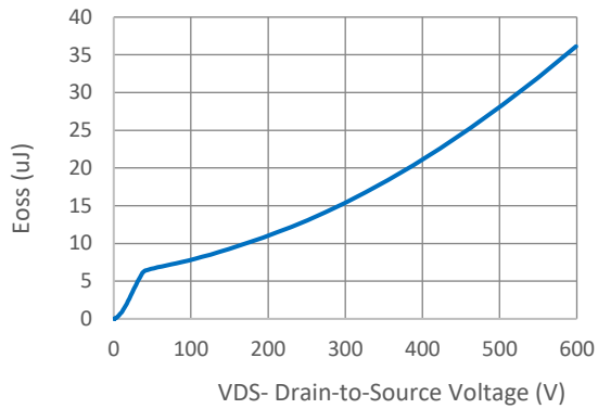
Fig.13 Typ. Coss Stored Energy
