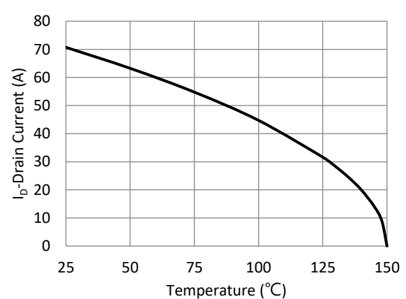
Fig.10 Drain Current vs. Case Temperature
