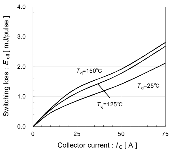
Switching loss vs. Collector current (typ.) V_{DC}=300\text{V}, V_{CC}=15\text{V}, \text{Resistive load}
