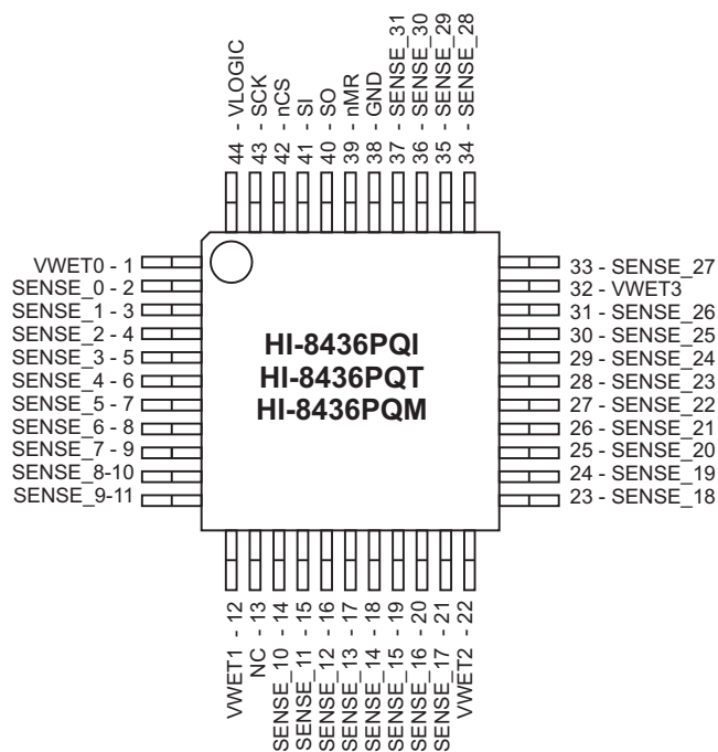
44 Pin Plastic Quad Flat Pack (PQFP) 10mm x 10mm
