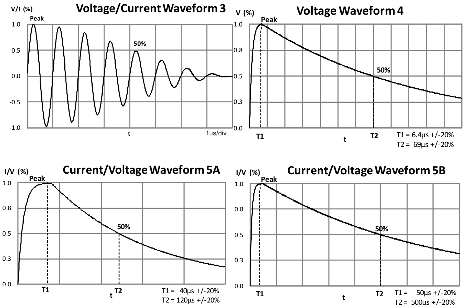
Figure 10. Lightning Waveforms
