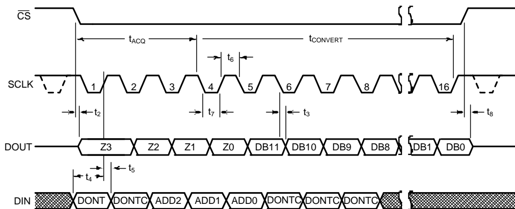
Figure 4. ADC78H90 Serial Timing Diagram
