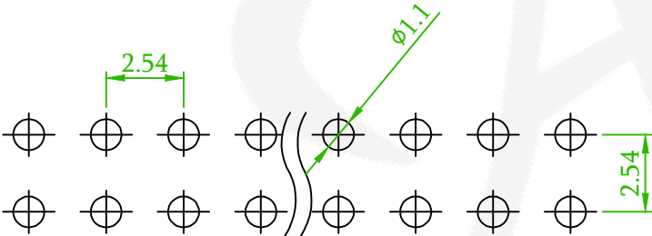
Recommended PCB Layout (PCB TOLERANCE ±0.1)
