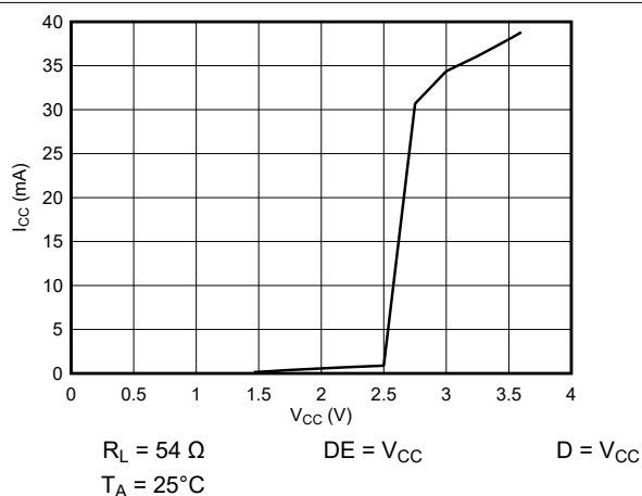
Figure 6-3. Supply Current vs Supply Voltage
