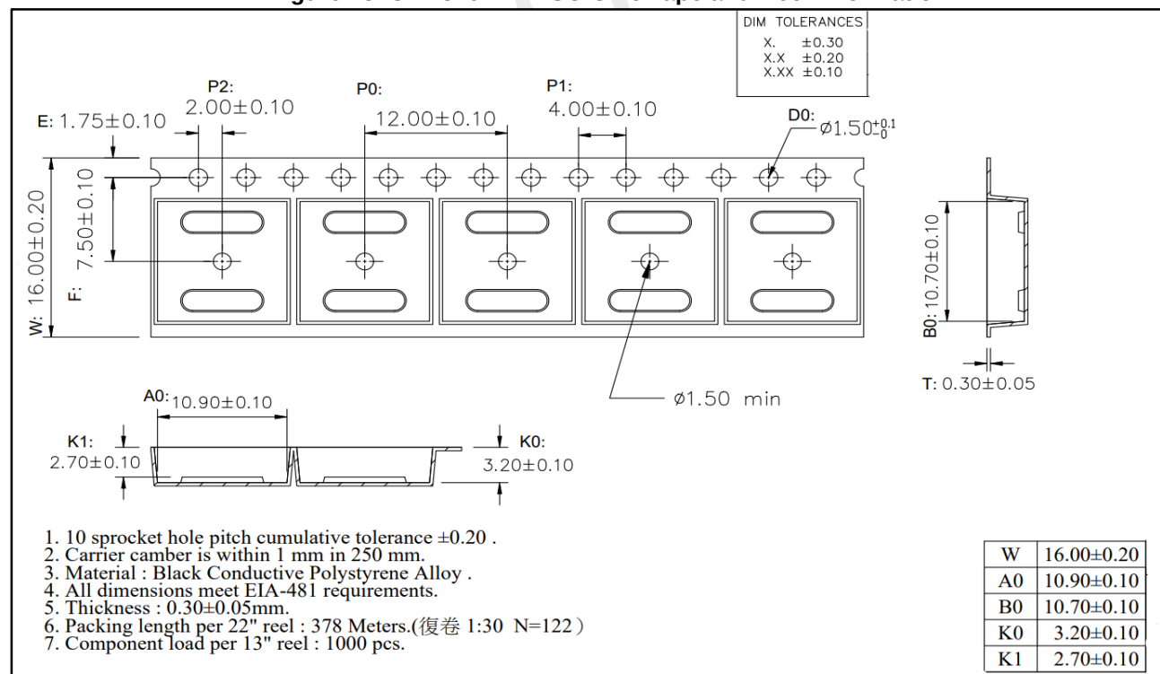
Figure 15. CMT826X WB SOIC-16 Tape and Reel Information
