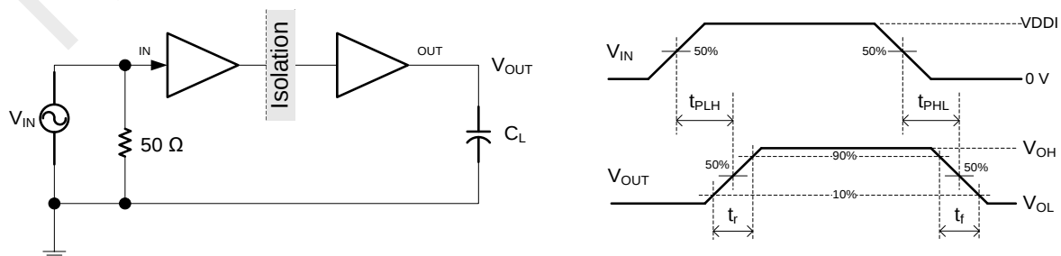
Figure 3. Switching Characteristics Test Circuit and Voltage Waveforms
