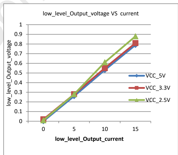
Figure 9-4. Low-Level Output Voltage vs. Low-Level Output Current ( T_A=25^{\circ}\text{C} )
