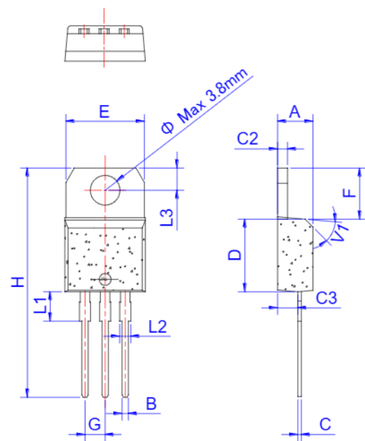
TO-220B Non-Ins
