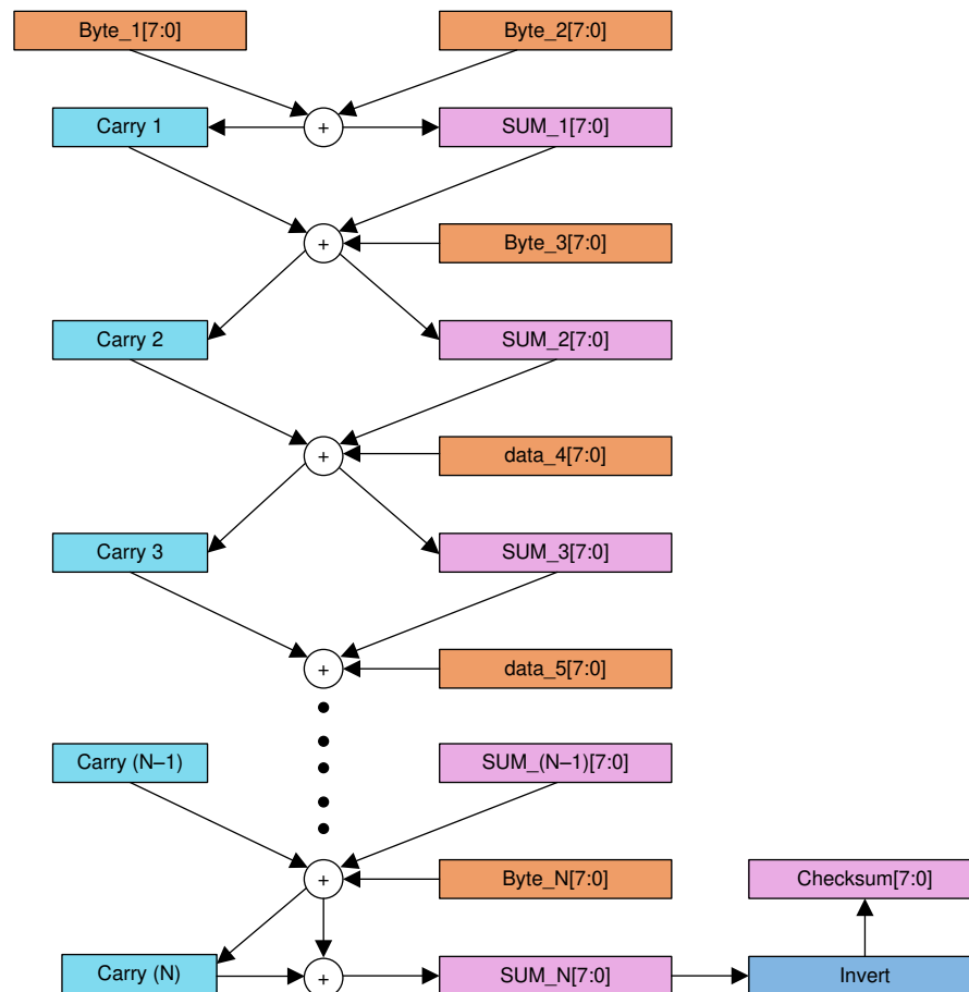
Figure 7-17. Checksum Calculation
