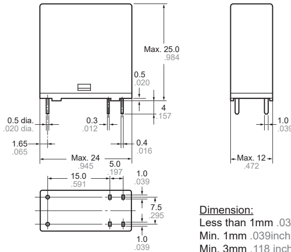
External dimensions
