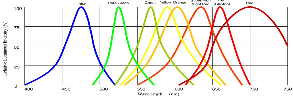
Spectral Distribution
