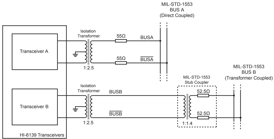
Figure 28. Bus Connection Example using HI-6139
