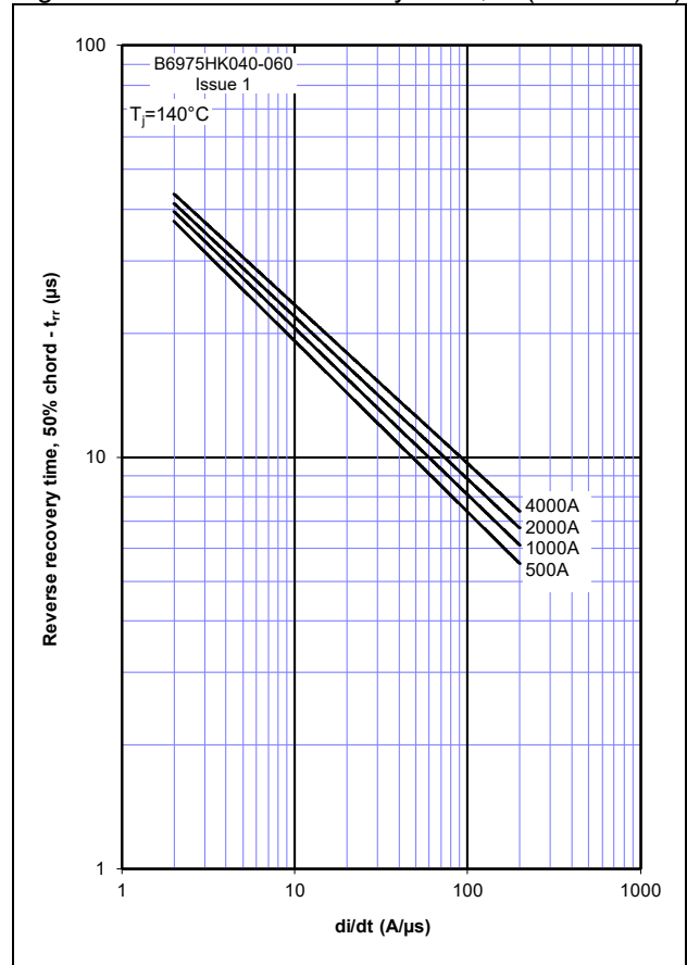
Figure 7 – Maximum Recovery Time, t_{rr} (50% chord)
