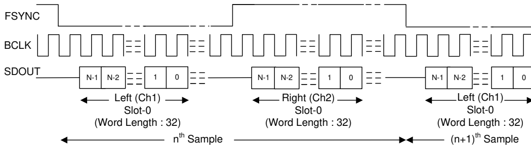
Figure 7-4. I 2 S Mode Protocol Timing (MD0 shorted to ground) in Target Mode
