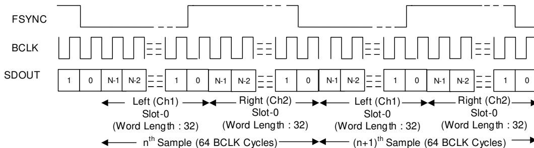
Figure 7-5. I 2 S Protocol Timing (MD0 shorted to AVDD) In Controller Mode
