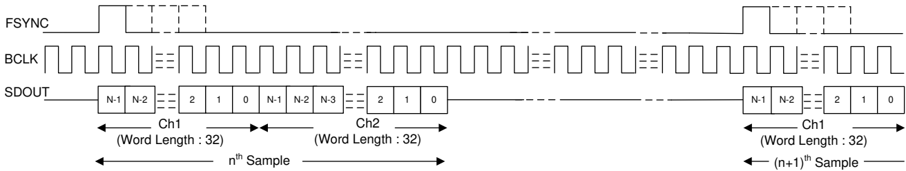
Figure 7-2. TDM Mode Protocol Timing (MD0 shorted to ground with 4.7K Ohms) In Target Mode
