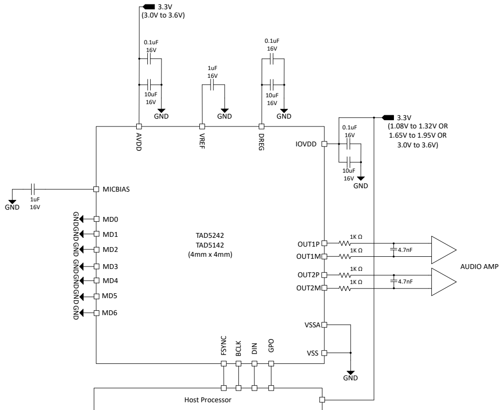
Figure 8-1. Stereo Lineout in Target I2S Mode Block Diagram
