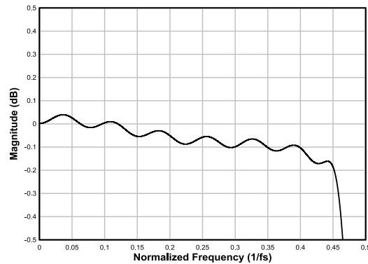
Figure 7-16. Linear Phase Interpolation Filter Pass-Band Ripple
