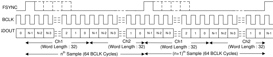
Figure 7-3. TDM Mode Protocol Timing (MD0 shorted to AVDD with 4.7K Ohms) In Controller Mode
