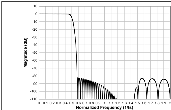
Figure 7-15. Linear Phase Interpolation Filter Magnitude Response
