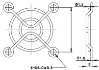
PFG-40 For 40mm Fan
