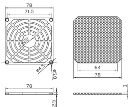
PFGF-80 For 80mm Fan
