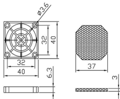
PFGF-40 For 40mm Fan
