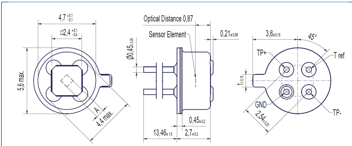
Figure 4 Mechanical Drawing of the TPD 1T 0623 (Drawing No.: 2/71830-0)
