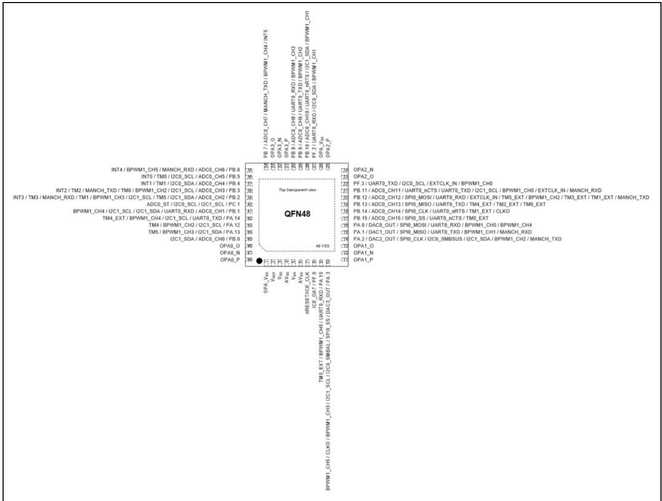
Figure 4.1-6 M091YD2AE QFN 48-pin Multi-function Pin Diagram
