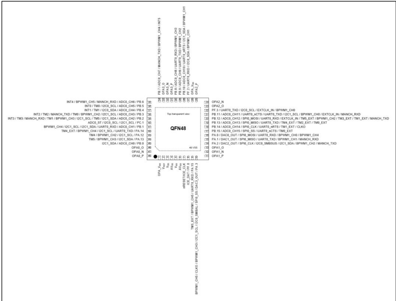
Figure 4.1-5 M091YC2AE QFN 48-pin Multi-function Pin Diagram
