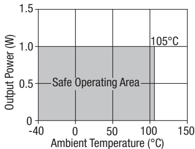
NMV0505TSAC & NMV0512TSC:
