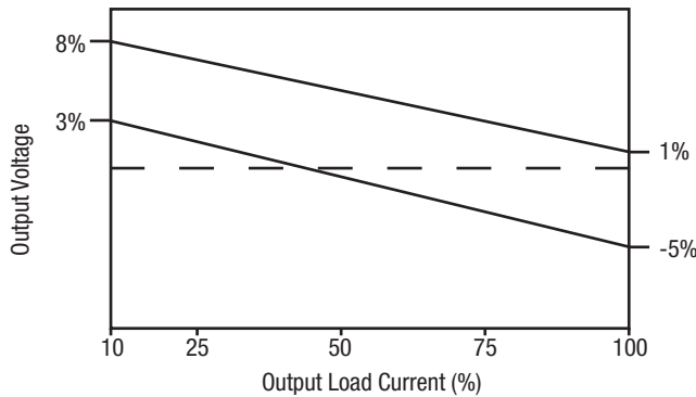
NMV0505TSAC
