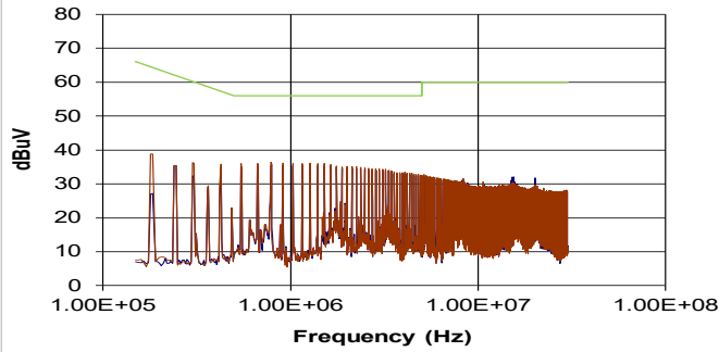
NMV0512TSC (Quasi-Peak)
