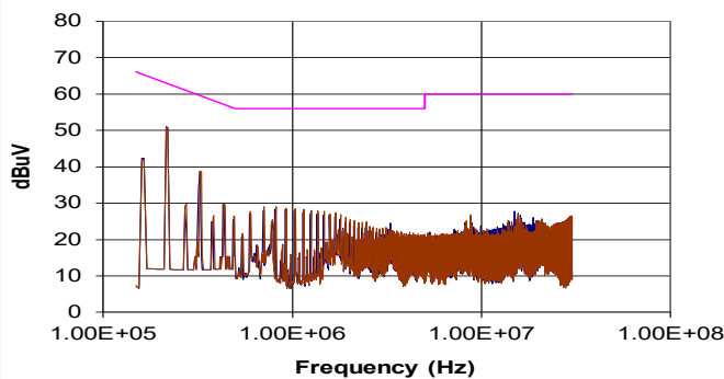
NMV0505TSAC (Quasi-Peak)
