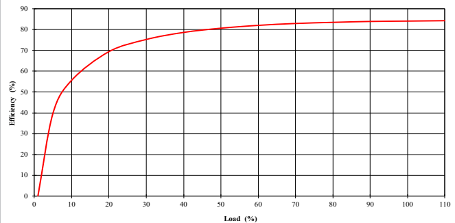
NMV0512TSC
