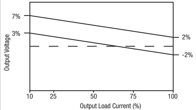
NMV0512TSC
