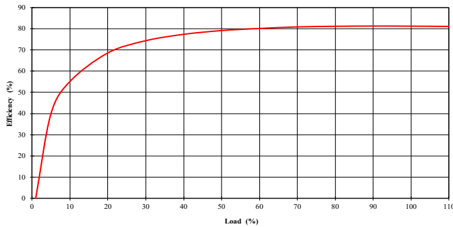
NMV0505TSAC
